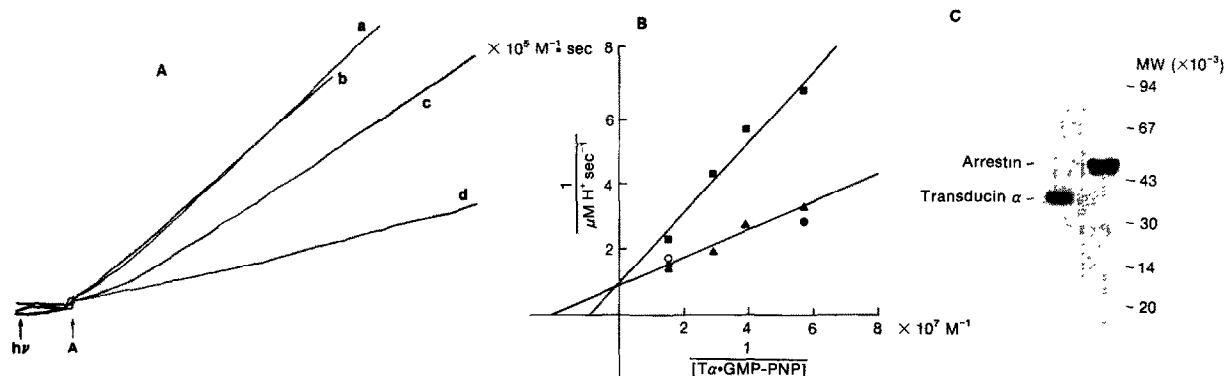
Fig.4. Activation of PDE by Tα·PNPs is competitively inhibited by arrestins in the presence of ATP. Representative pH records in panel A, double reciprocal plot of data in panel B, gels of purified proteins in panel C. (A) 10 μg purified arrestin and/or 100 μM ATP added, when indicated, prior to a flash that bleached a 1.6 \times 10^{-5} fraction of rhodopsin. Curves: (a) no prior additions, 2 μg Tα·GMP-PNP injected into cuvette at A; (b) 100 μM ATP added prior to flash, 2 μg Tα·GMP-PNP added at A; (c) no prior additions, 1 μg Tα·GMP-PNP added at A; (d) 10 μg arrestin and 100 μM ATP added prior to flash, 1 μg Tα·GMP-PNP added at A. Reaction buffer, rhodopsin concentration, temperature and volume as in fig.2. (B) Arrestin (10 μg) + 100 μM ATP + Tα·GMP-PNP (■); Tα·GMP-PNP (▲); Tα·GMP-PNP + arrestin (10 μg) (●); Tα·GMP-PNP + 100 μM ATP (○). (C) SDS-PAGE of purified proteins used in this figure, panels A and B, and in figs 1-3. Left lane, enriched Tα·GMP-PNP; right lane, purified arrestin prepared as in section 2.
